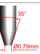
blunt taper indenter
